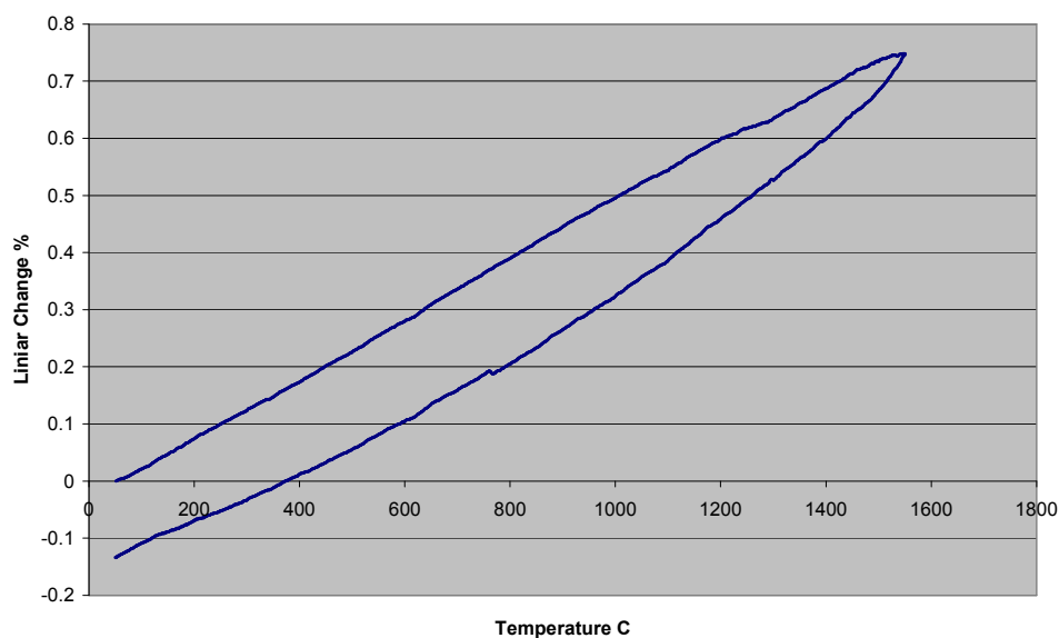
Thermal Expansion 330
