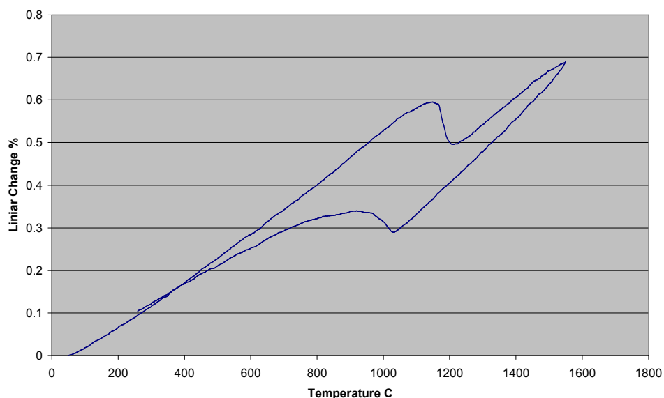
Thermal Expansion 300
